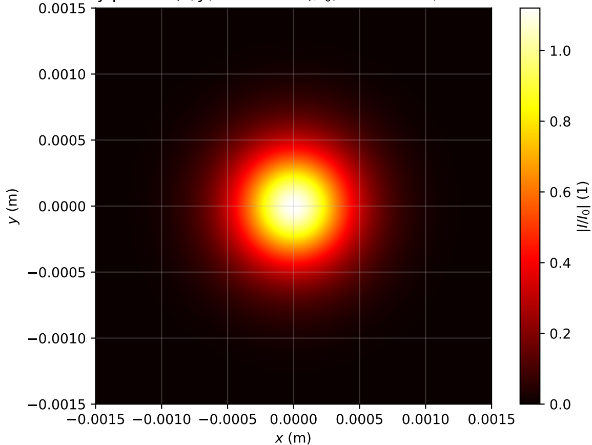
Intensity profile I(x, y, z = 0.955m)/I_0 , P_{in}=0.6P_{cr} , artificial time
